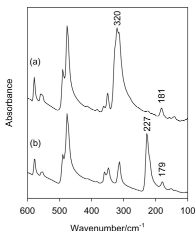
Figure 3. Far-IR spectra of [(\text{Bn}_3\text{P})\text{AuX}] ; (a) \text{X} = \text{Cl} ; (b) \text{X} = \text{Br} .
