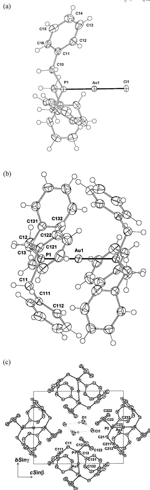
Figure 1. (a) Molecule 1 of [(\text{Bn}_3\text{P})\text{AuCl}] (the other two molecules and those of the isomorphous bromide analogue are similar); (b) Cation 1 of [\text{Au}(\text{PBn}_3)_2]\text{Cl} \cdot \text{H}_2\text{O} (the other cation and that of the \text{BF}_4 salt are similar); (c) Unit cell contents of [\text{Au}(\text{PBn}_3)_2]\text{Cl} \cdot \text{H}_2\text{O} , projected down the a axis.
