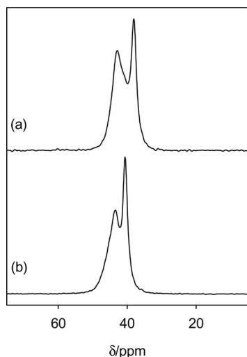
Figure 5. ^{31}\text{P} CP MAS spectra of [(\text{Bn}_3\text{P})\text{AuX}] at B = 11.7\text{ T} , (a) \text{X} = \text{Cl} , (b) \text{X} = \text{Br} .
