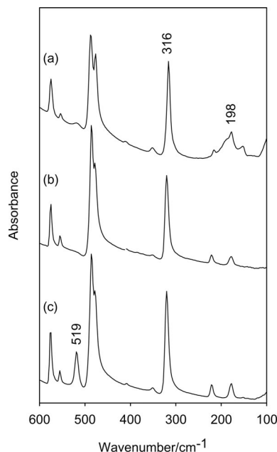
Figure 4. Far-IR spectra of [\text{Au}(\text{PBn}_3)_2]\text{X} , (a) \text{X} = \text{Cl}\cdot 2\text{H}_2\text{O} ; (b) \text{X} = \text{I} , (c) \text{X} = \text{BF}_4 .
