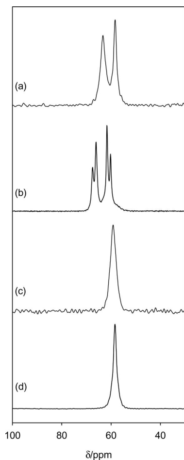
Figure 6. ^{31}\text{P} CP MAS spectra of [\text{Au}(\text{PBn}_3)_2]\text{X} at B = 11.7\text{ T} ; (a) \text{X} = \text{Cl}\cdot\text{H}_2\text{O} ; (b) \text{X} = \text{Cl}\cdot 2\text{H}_2\text{O} ; (c) \text{X} = \text{I} ; (d) \text{X} = \text{BF}_4 .
