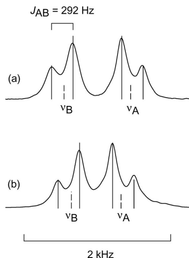
Figure 7. ^{31}\text{P} CP MAS spectra of [\text{Au}(\text{PBn}_3)_2]\text{Cl}\cdot 2\text{H}_2\text{O} , (a) B = 9.4 T; (b) B = 7.0 T. The superimposed stick plots are the calculated AB spectra for the two fields, with \delta_{\text{A}} = 60.9 , \delta_{\text{B}} = 66.6 , J_{\text{AB}} = 292 Hz.
