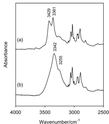
Figure 2. IR spectra of (a) [Au(PBn 3 ) 2 ]Cl·H 2 O; (b) [Au(PBn 3 ) 2 ]Cl·2H 2 O in the 4000–2500 cm −1 region. The bands assigned to ν(OH) modes are labelled with their wavenumbers.
